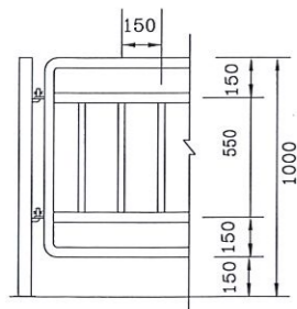
HEIGHT DIMENSION OF RAILING
